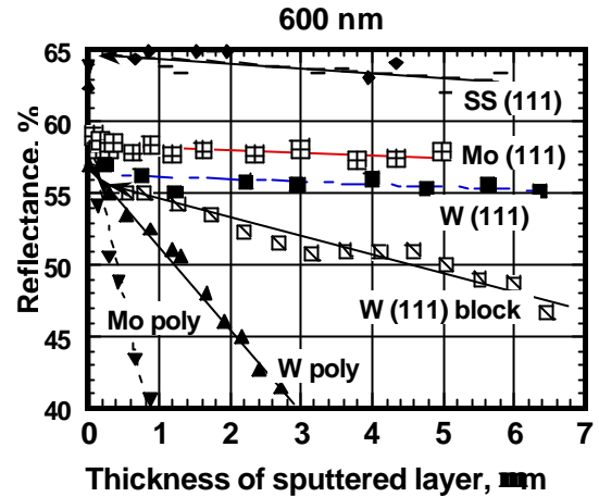
FIG.2. Reflectance of SS single crystal, W and Mo mirrors of different structure (polycrystal, block single crystal and single crystals with (111) planes of orientation) at 600 nm depending on the thickness of the layer eroded due to bombardment by ions of deuterium plasma.
