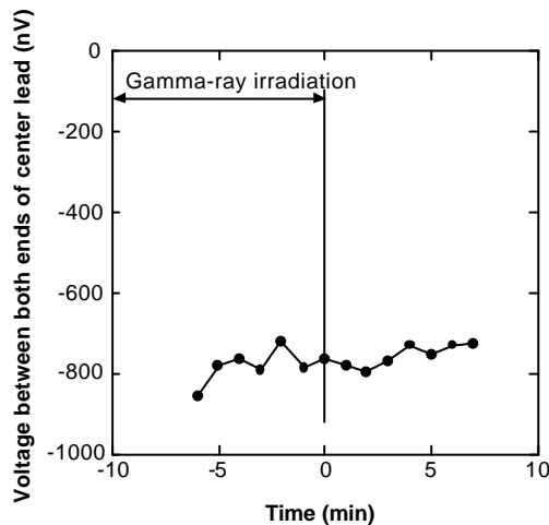
FIG.1. Time evolution of the voltage across a coil measured in a test rig ( ^{60}\text{Co} , 4 Gy/s). The upper limit of 50 nV of differential voltage change at the transition translates to > 800 s of pulse length under ITER conditions for this (smaller than planned) test coil. More sensitive tests are planned. (Adapted from [6]).
